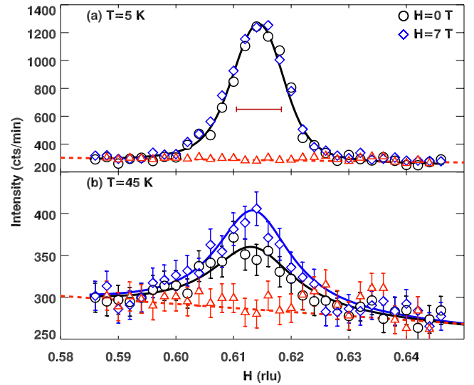
FIG. 2. (Color online) Selected elastic scans along \mathbf{Q} = (H, 0.5, 0) in zero field (open circles) and 7 T field (diamonds) at 5 and 45 K. Solid lines are guides for the eyes. The triangles show 55 K data as the background, as indicated by the dashed lines. The horizontal line in (a) shows the instrumental resolution (FWHM). Error bars represent the square root of the counts, and those smaller than the symbols are absent.
