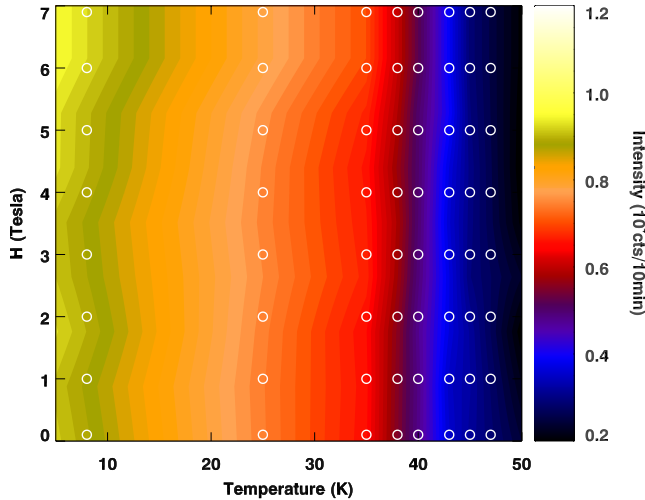
FIG. 3. (Color online) Contour map of the spin-order peak (0.615, 0.5, 0) intensity as a function of temperature and magnetic field. Circles indicate the fields and temperatures at which the measurements were performed.
